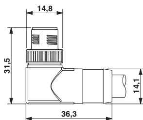
Plugue M12 SPEEDCON, angular, blindado
